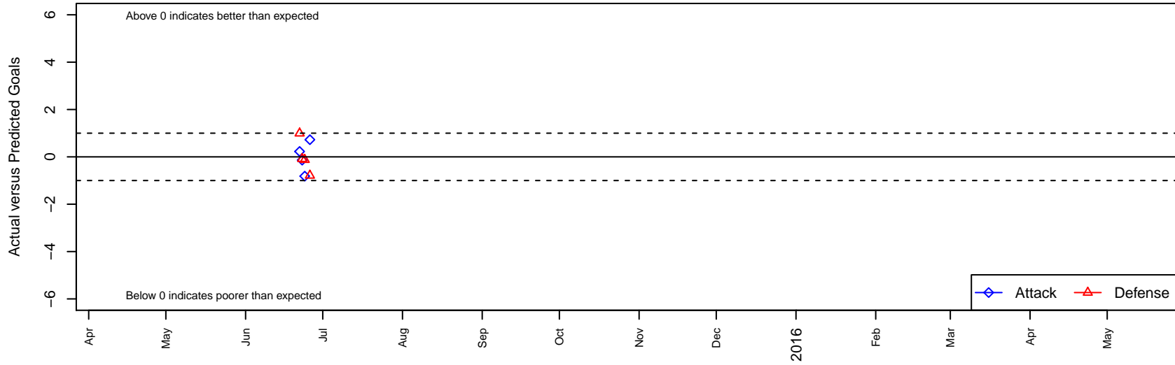
SC Del Sol 03 Lester G02 Dots are actual minus expected GF (blue circles) and GA (red triangles). Blue line is smoothed change in attack strength. Red is smoothed change in defense strength.
